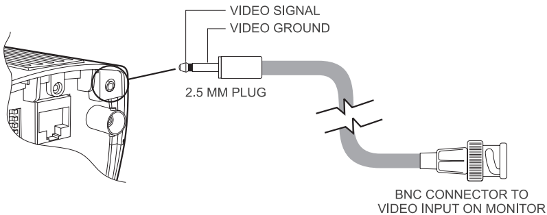
Figure 6. Service Connector
